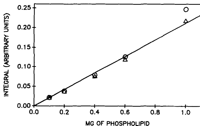
Fig. 4. Relationship between total phospholipid and the integral of the Mn^{2+} -quenched N-methyl choline signal from Fig. 3. Data are presented for vesicles alone (O-O) and a mixture of normal lipoproteins and vesicles ( \Delta - \Delta ).
