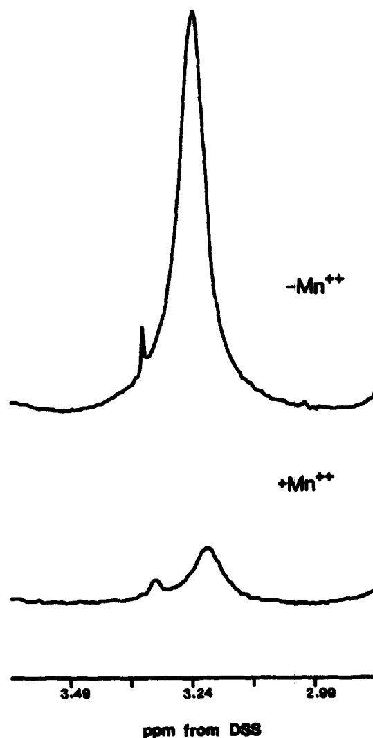
Fig. 5. Two hundred MHz ^1H -NMR spectra of the N-methyl choline region of 4.0 mg/ml phospholipid in the total lipoproteins isolated from an LCAT-deficient patient in the absence (top) and presence (bottom) of 1 mM MnSO_4 .
