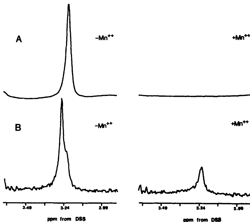
Fig. 2. Two hundred MHz 1 H-NMR spectrum of N-methyl choline region of (A) normal lipoproteins and (B) egg phosphatidylcholine-cholesterol vesicles. The spectra on the right are normal lipoproteins (top) and vesicles (bottom) in the presence of 1 mM MnSO 4 . The concentration of phospholipid in normal lipoproteins and the vesicles used was 4.0 and 0.5 mg/ml, respectively.
