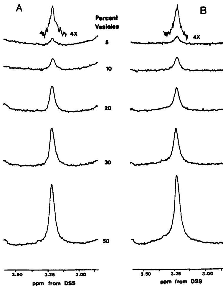
Fig. 3. Two hundred MHz ^1H -NMR spectra of N-methyl choline region of a mixture of egg phosphatidylcholine-cholesterol vesicles plus total lipoproteins (A) and egg phosphatidylcholine-cholesterol vesicles (B) in the presence of 1 mM MnSO_4 . The mixture of lipoproteins contained in indicated amounts of vesicular phospholipid. (B) is the Mn^{2+} -quenched signal of equivalent amounts of vesicles in the absence of lipoproteins.
