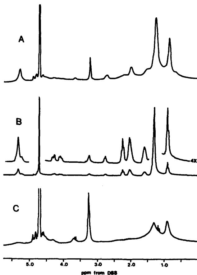
Fig. 1. Two hundred MHz 1 H-NMR spectra of (A) normal lipoproteins; (B) LCAT-deficient plasma lipoproteins; and (C) egg phosphatidylcholine-cholesterol 55:45 (mol %) unilamellar vesicles.
